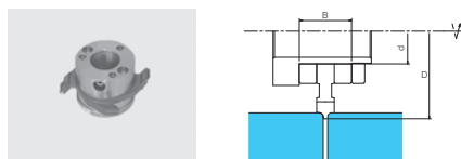
2 nd horizontal profiling top side
