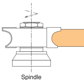
Clockwise rotation
